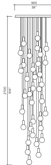
Model Size 130 Ref. # 36SM.07.87_ _ _ _ _ Bulb 36 x 4W LED 3200K, 360Lm/ea.
